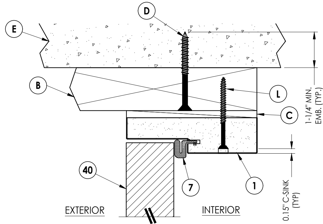
3 VERTICAL CROSS SECTION 3 Outswing shown (Inswing similar)
