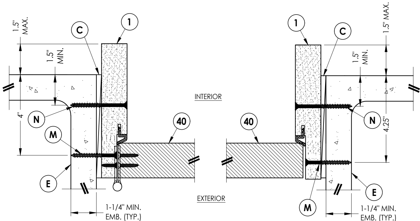
4 7 HORIZONTAL CROSS SECTION Shown Direct to Masonry Outswing only w/ 6-9/16" jamb
